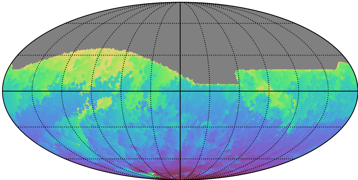
ddf_acor_sf30_lsf40_lsr50_v3.4_10yrs All sky z band: Min HA
