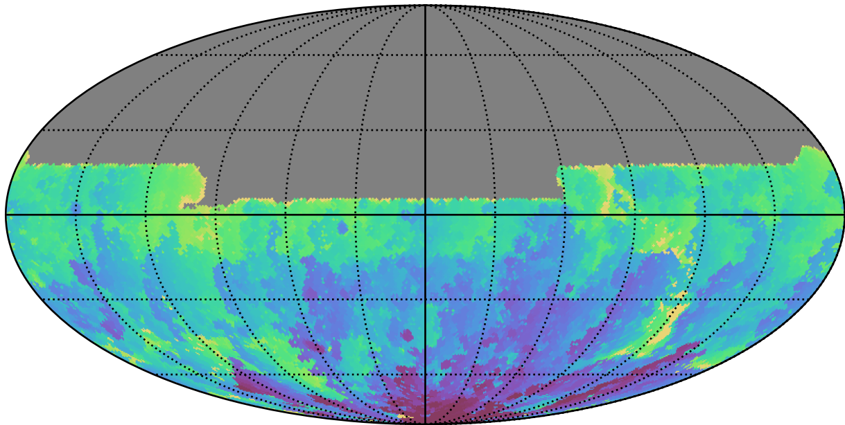
ddf_acor_sf30_lsf40_lsr50_v3.4_10yrs All sky u band: Min HA
