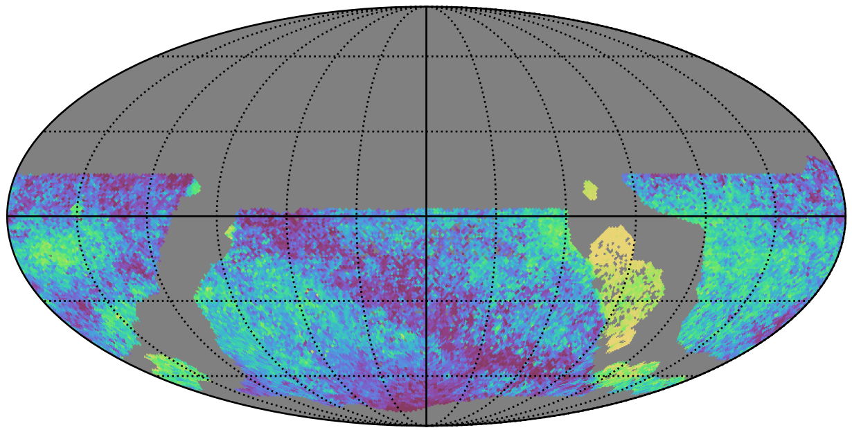
ddf_acor_sf30_lsf40_lsr50_v3.4_10yrs WFD all bands: Median skyBrightness
