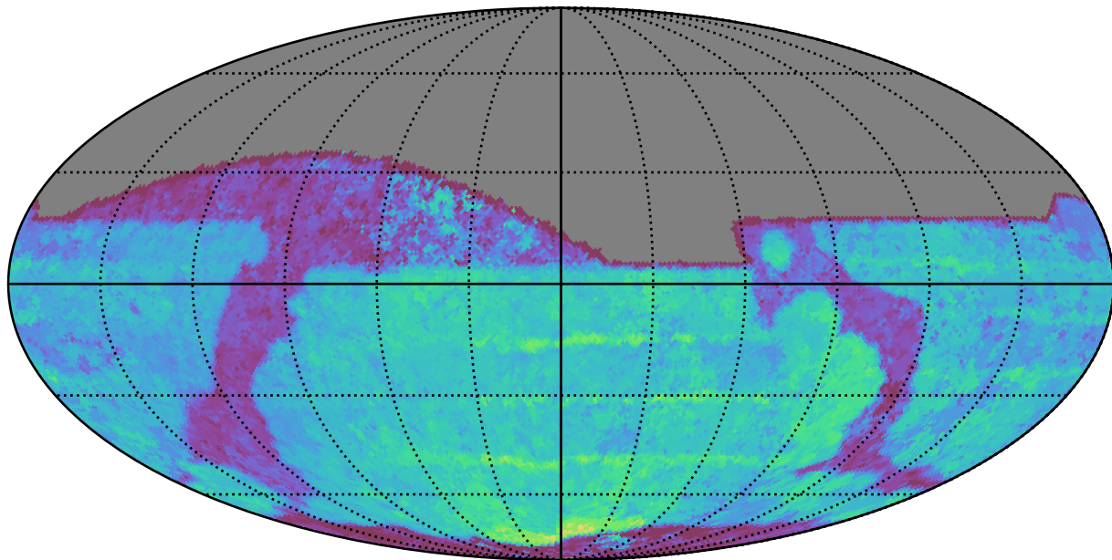
ddf_acor_sf30_lsf40_lsr50_v3.4_10yrs All sky z band: Median Season Length
