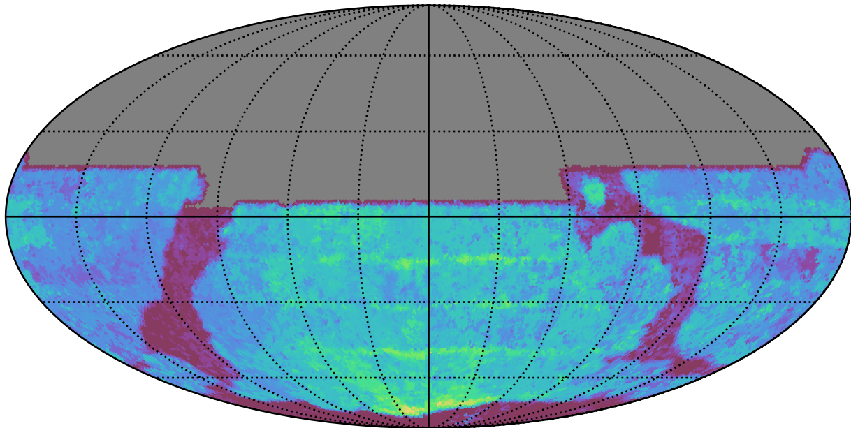
ddf_acor_sf30_lsf40_lsr50_v3.4_10yrs All sky y band: Median Season Length
