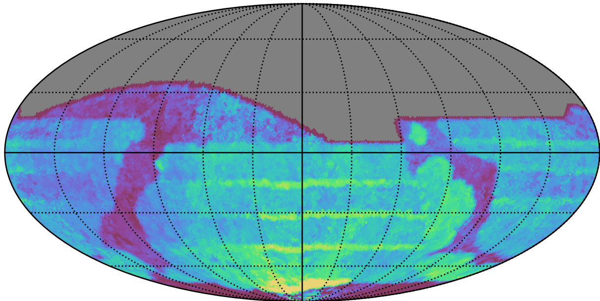
ddf_acor_sf30_lsf40_lsr50_v3.4_10yrs All sky all bands: Median Season Length
