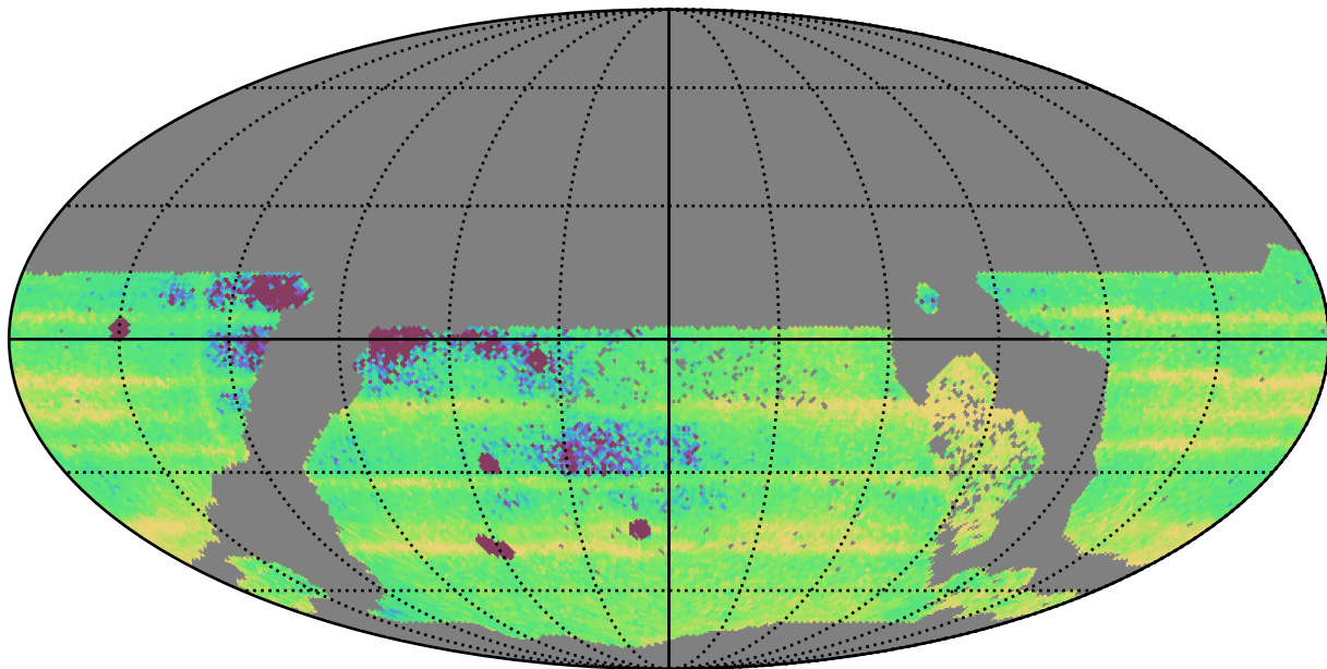
ddf_acor_sf30_lsf40_lsr50_v3.4_10yrs WFD: Median Intra-Night Gap
