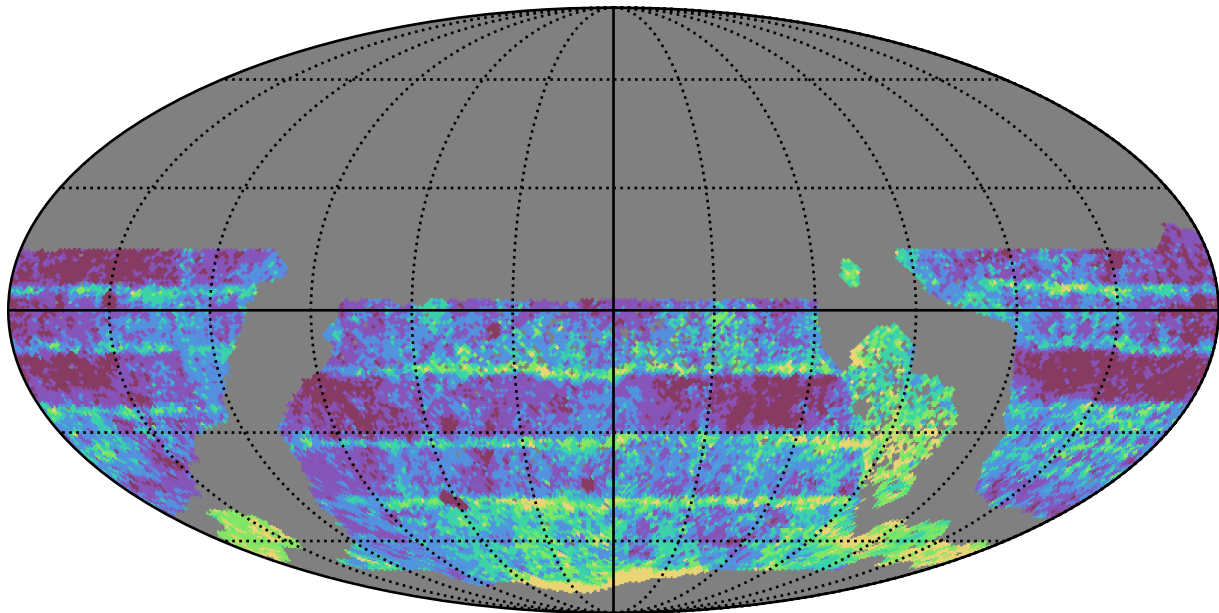
ddf_acor_sf30_lsf40_lsr50_v3.4_10yrs WFD r band: Median Inter-Night Gap
