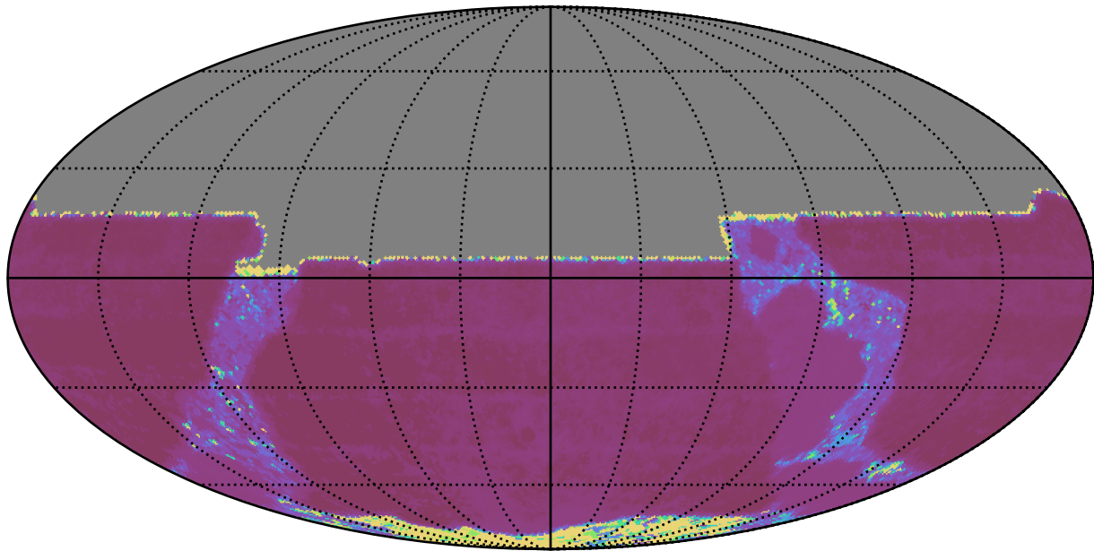
ddf_acor_sf30_lsf40_lsr50_v3.4_10yrs All sky y band: Median Inter-Night Gap
