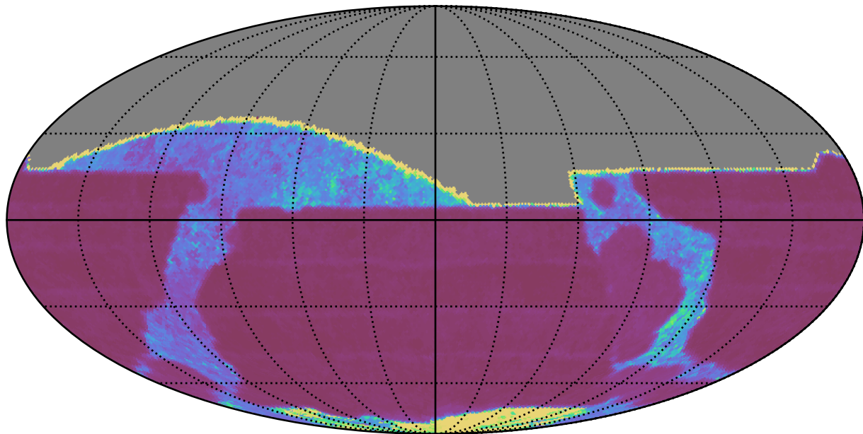
ddf_acor_sf30_lsf40_lsr50_v3.4_10yrs All sky i band: Median Inter-Night Gap
