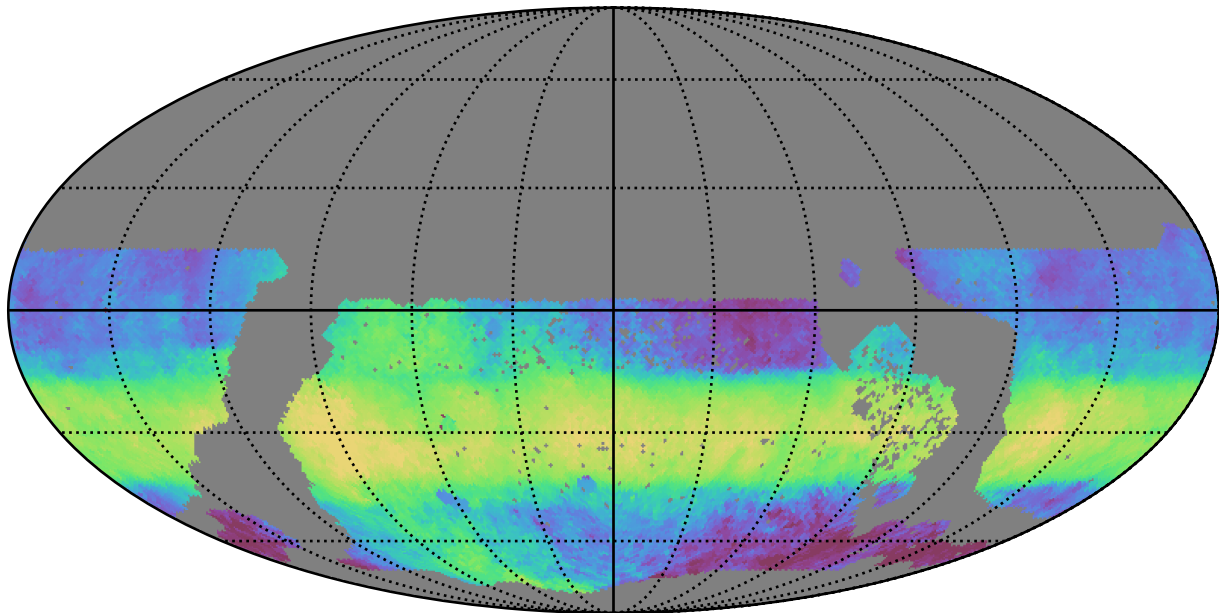
ddf_acor_sf30_lsf40_lsr50_v3.4_10yrs WFD z band: Median HA
