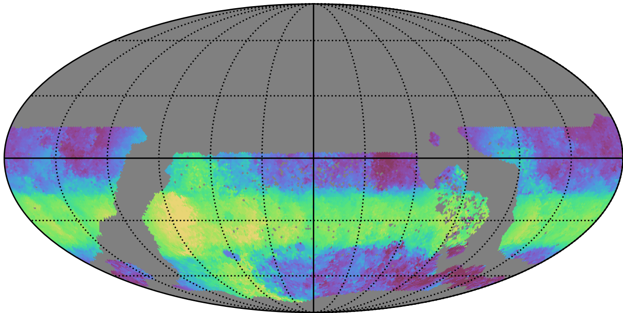
ddf_acor_sf30_lsf40_lsr50_v3.4_10yrs WFD u band: Median HA
