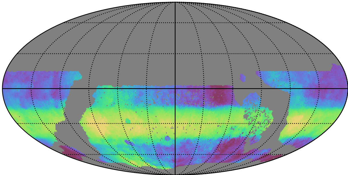
ddf_acor_sf30_lsf40_lsr50_v3.4_10yrs WFD r band: Median HA
