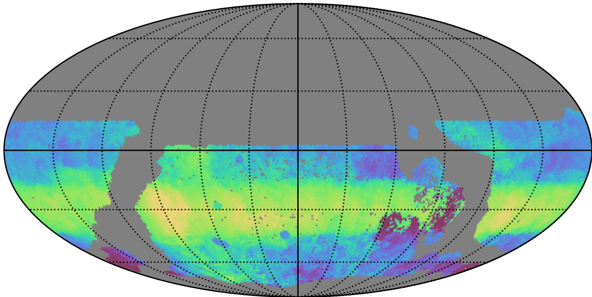
ddf_acor_sf30_lsf40_lsr50_v3.4_10yrs WFD g band: Median HA
