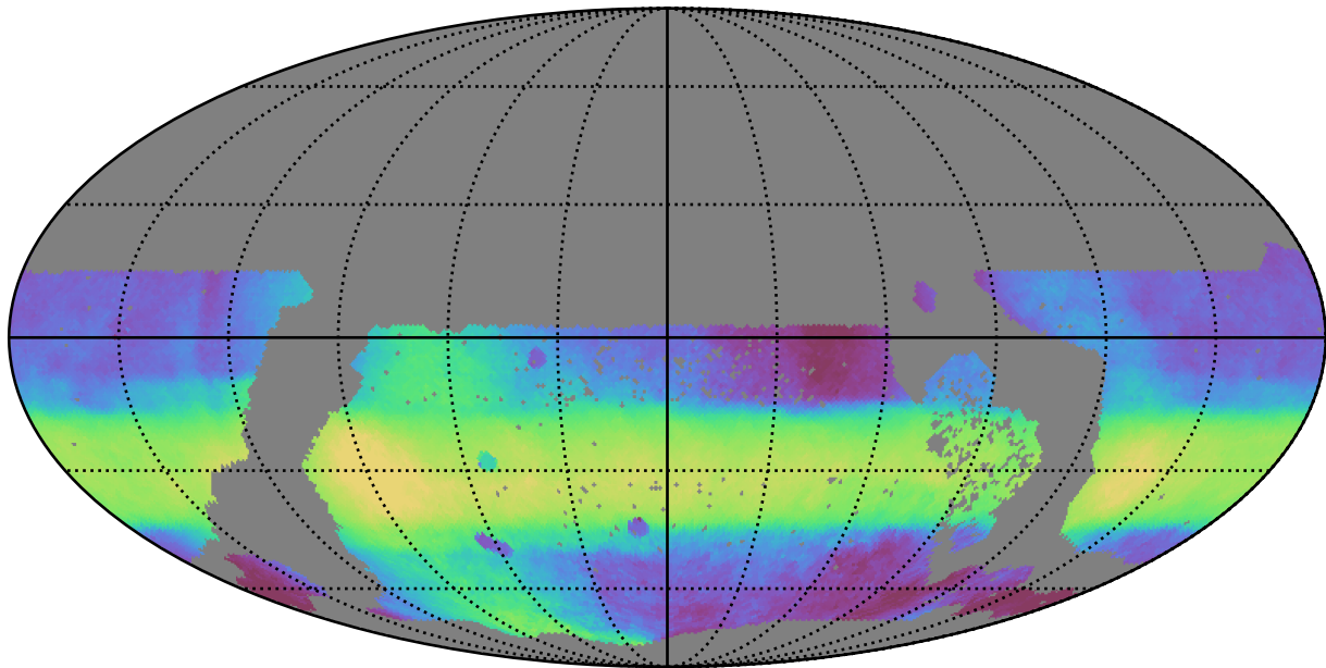
ddf_acor_sf30_lsf40_lsr50_v3.4_10yrs WFD all bands: Median HA
