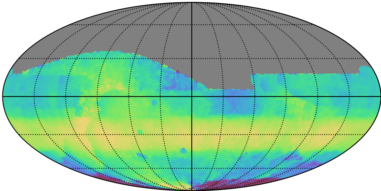
ddf_acor_sf30_lsf40_lsr50_v3.4_10yrs All sky i band: Median HA
