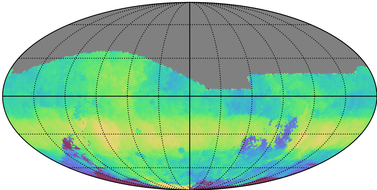
ddf_acor_sf30_lsf40_lsr50_v3.4_10yrs All sky g band: Median HA
