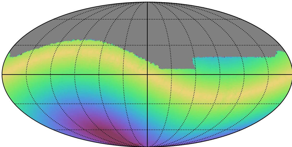
ddf_acor_sf30_lsf40_lsr50_v3.4_10yrs All sky r band: Max solarElong
