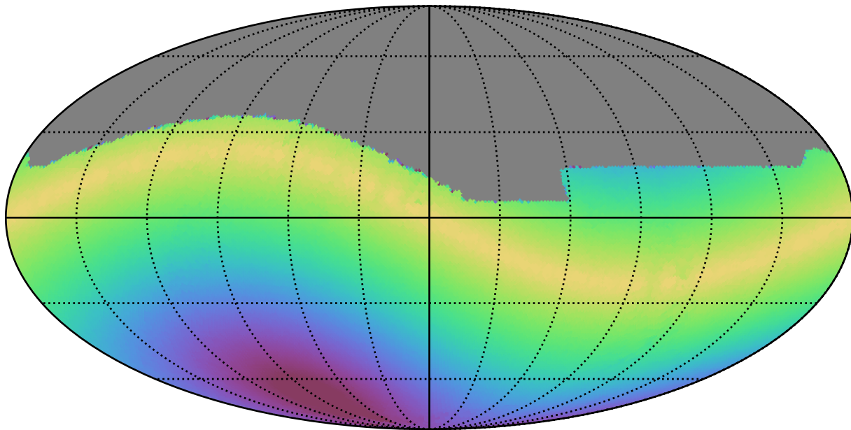
ddf_acor_sf30_lsf40_lsr50_v3.4_10yrs All sky i band: Max solarElong
