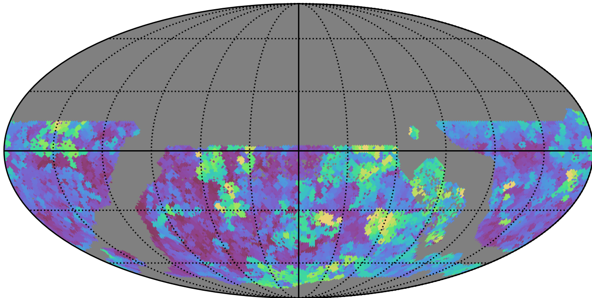
ddf_acor_sf30_lsf40_lsr50_v3.4_10yrs WFD g band: Max seeingEff
