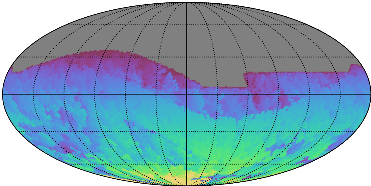
ddf_acor_sf30_lsf40_lsr50_v3.4_10yrs All sky z band: Max HA
