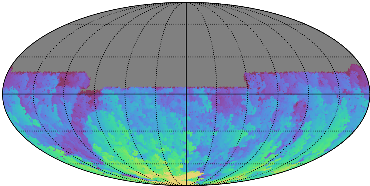
ddf_acor_sf30_lsf40_lsr50_v3.4_10yrs All sky u band: Max HA
