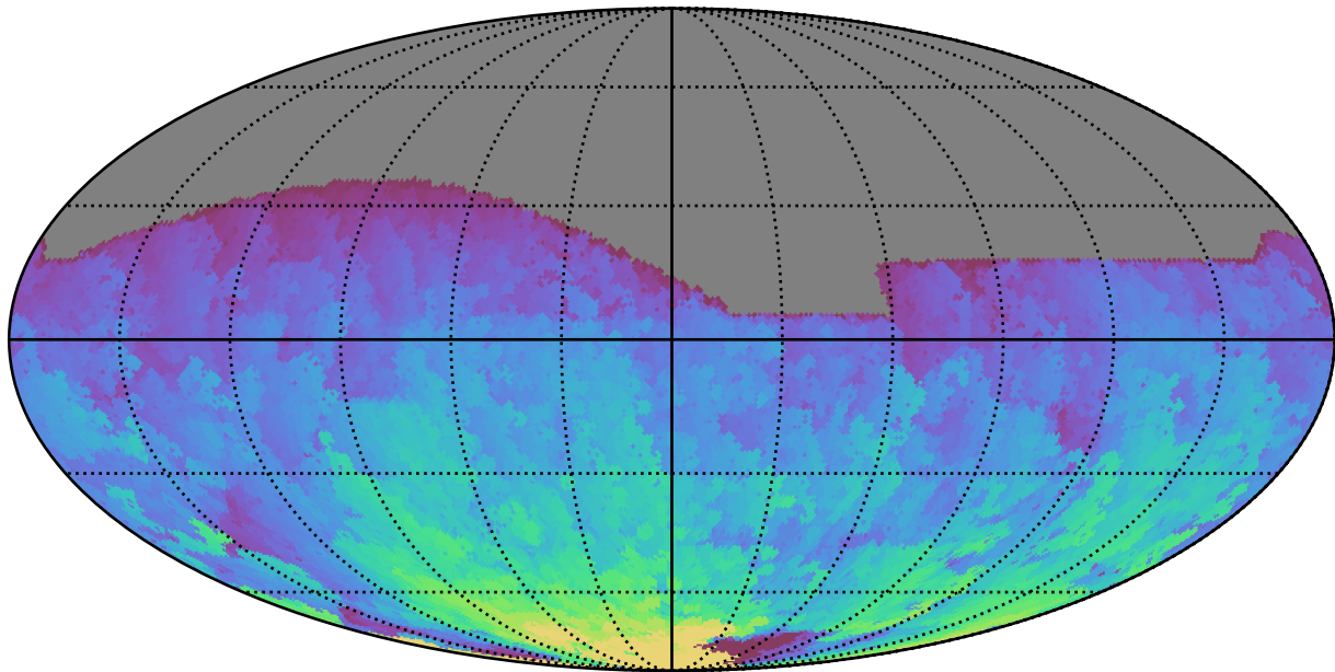
ddf_acor_sf30_lsf40_lsr50_v3.4_10yrs All sky r band: Max HA
