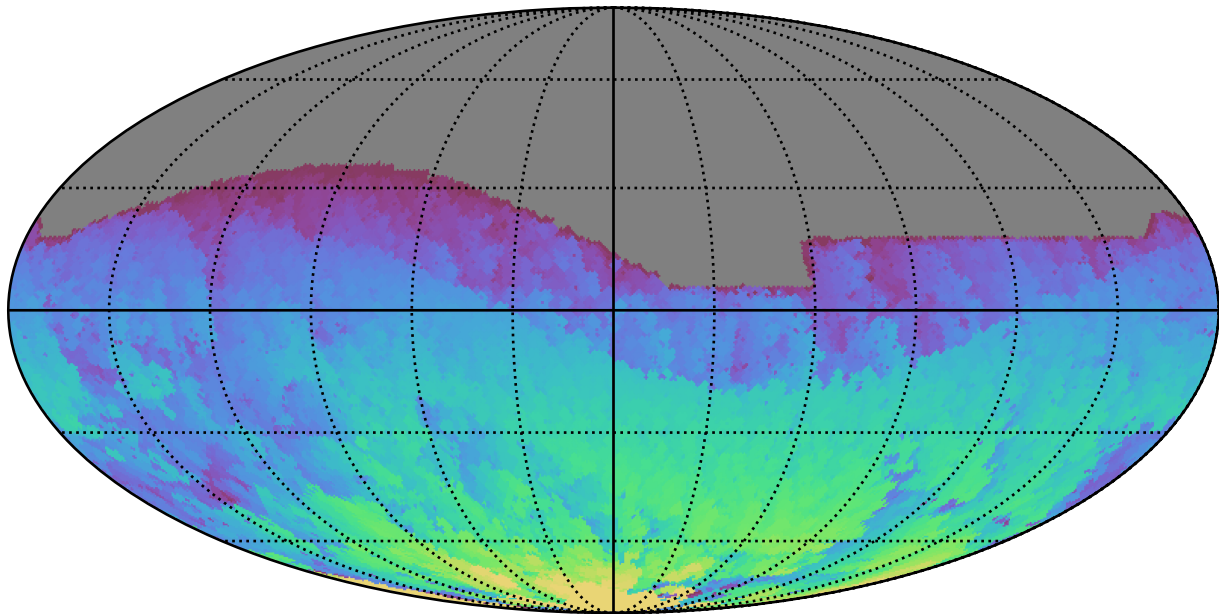
ddf_acor_sf30_lsf40_lsr50_v3.4_10yrs All sky i band: Max HA
