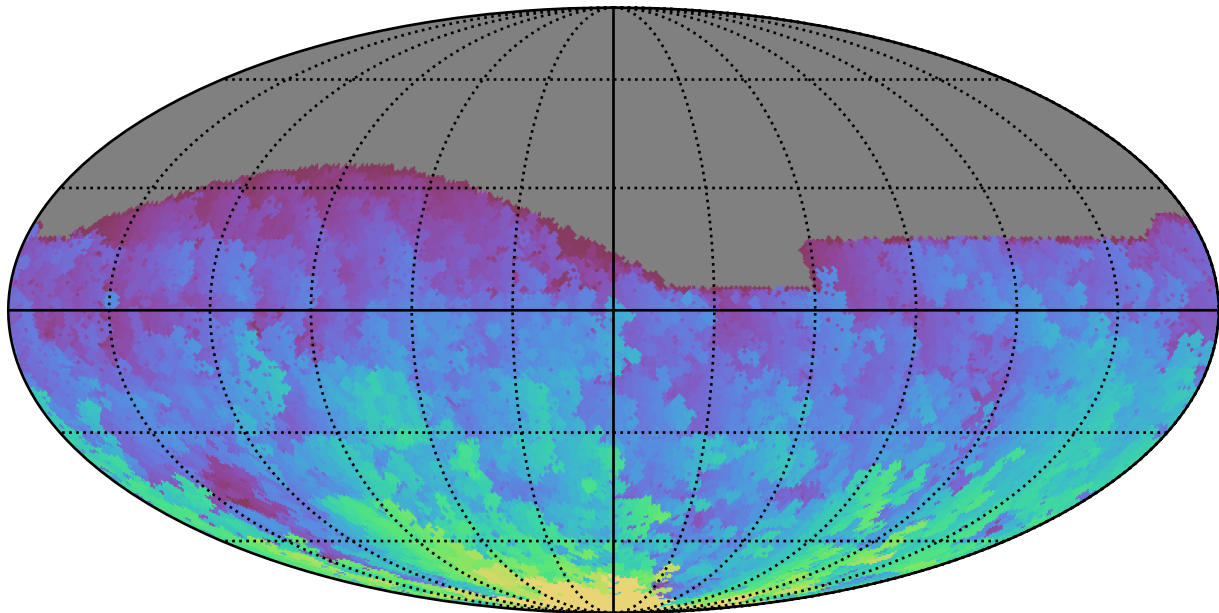
ddf_acor_sf30_lsf40_lsr50_v3.4_10yrs All sky g band: Max HA
