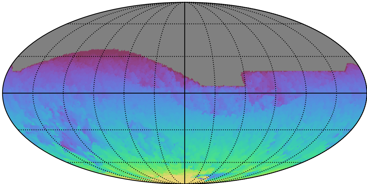
ddf_acor_sf30_lsf40_lsr50_v3.4_10yrs All sky all bands: Max HA
