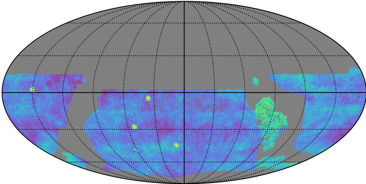
ddf_acor_sf30_lsf40_lsr50_v3.4_10yrs gri WFD: Fraction of visits in pairs (20-90 min)
