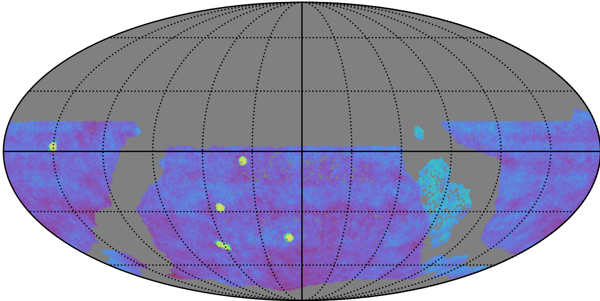
ddf_acor_sf30_ls40_lsr50_v3.4_10yrs gri WFD: Fraction of visits in pairs (10-60 min)
