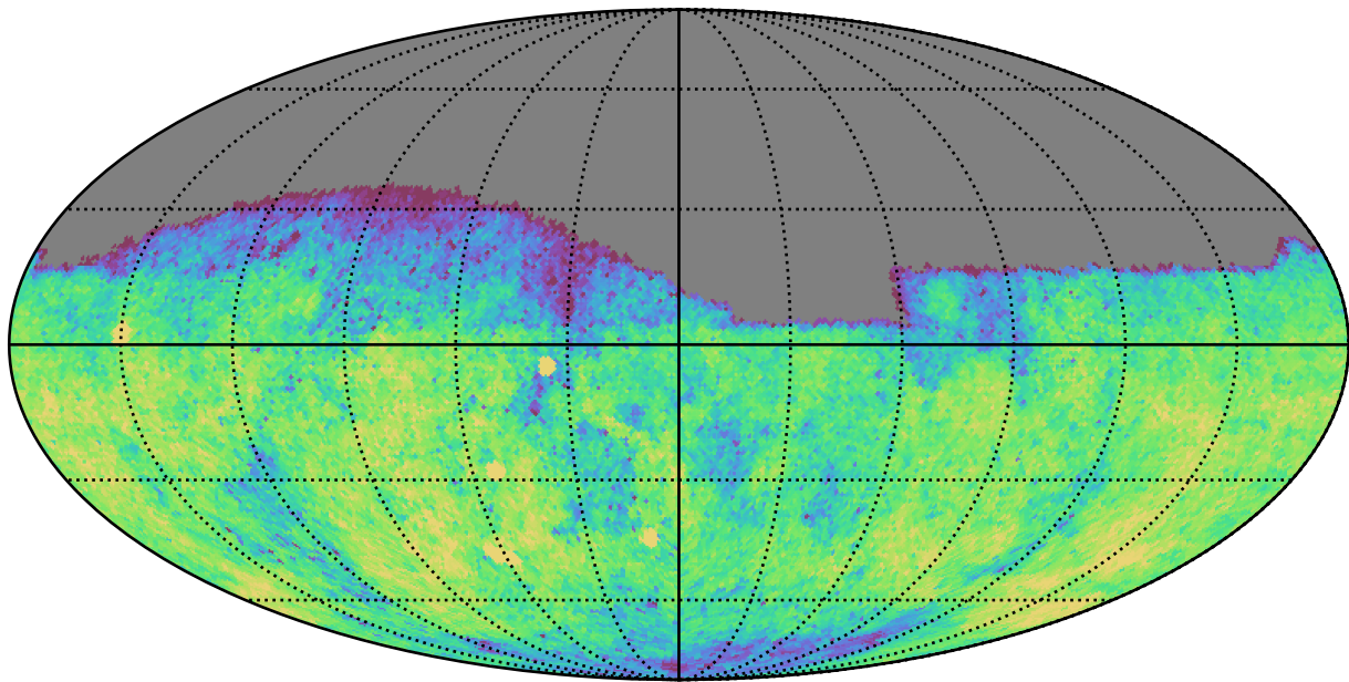
ddf_acor_sf30_lsf40_lsr50_v3.4_10yrs Yr 1 g band: CoaddM5
