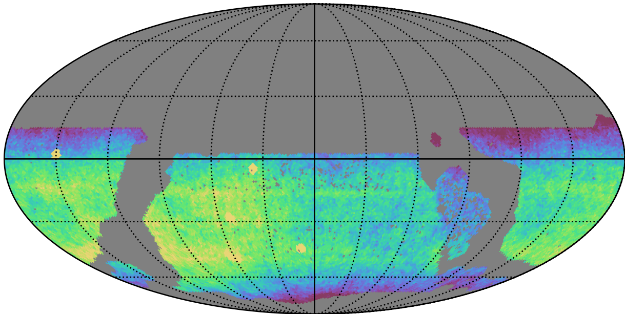
ddf_acor_sf30_lsf40_lsr50_v3.4_10yrs WFD z band: CoaddM5
