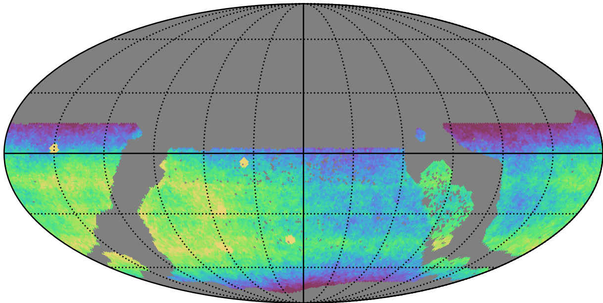
ddf_acor_sf30_lsf40_lsr50_v3.4_10yrs WFD r band: CoaddM5
