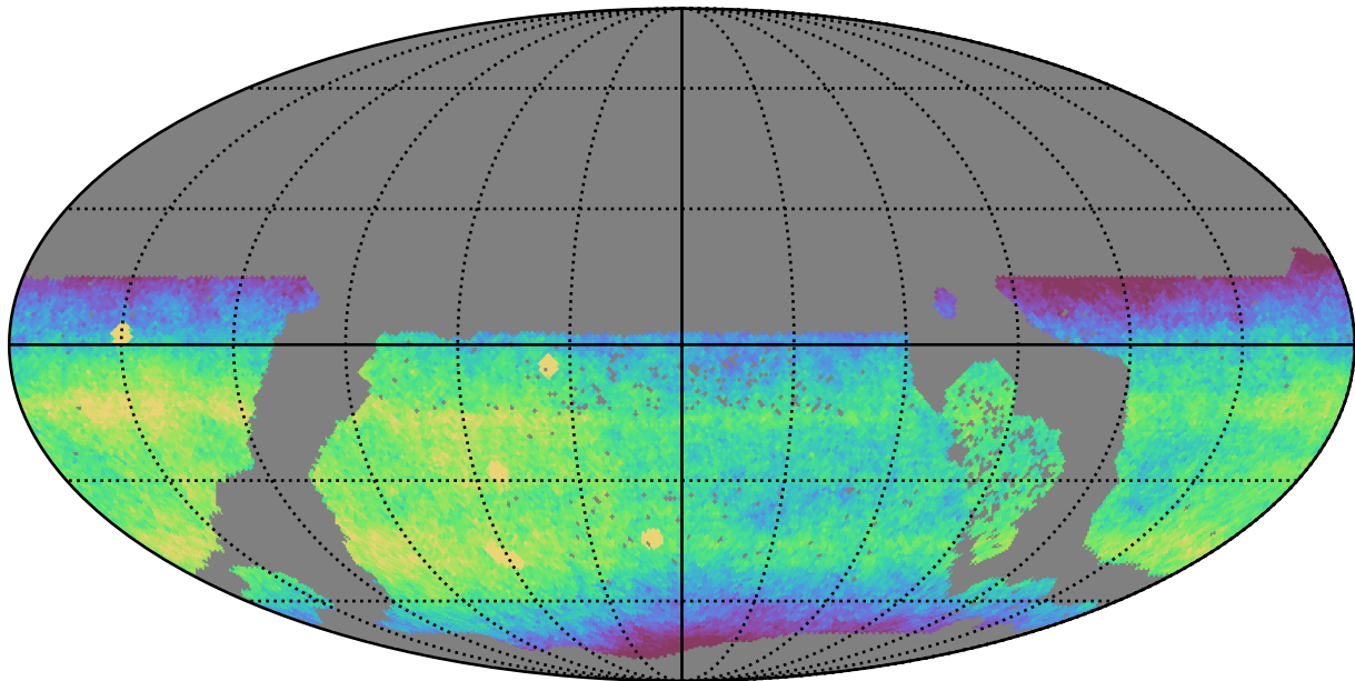
ddf_acor_sf30_lsf40_lsr50_v3.4_10yrs WFD i band: CoaddM5
