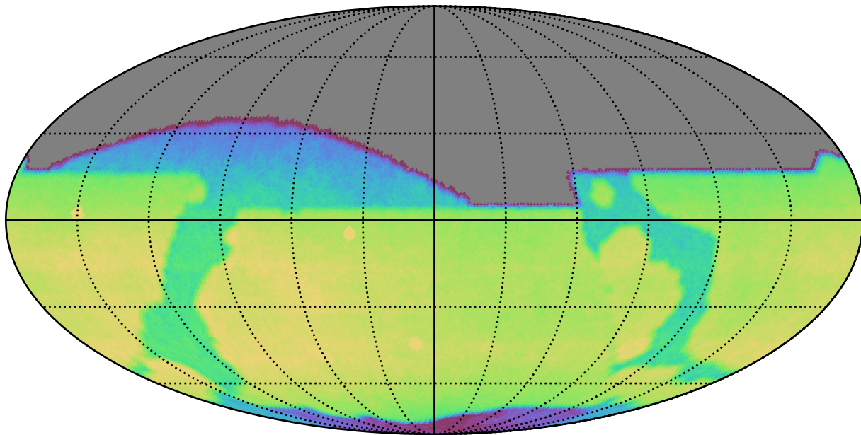
ddf_acor_sf30_lsf40_lsr50_v3.4_10yrs All sky r band: CoaddM5
