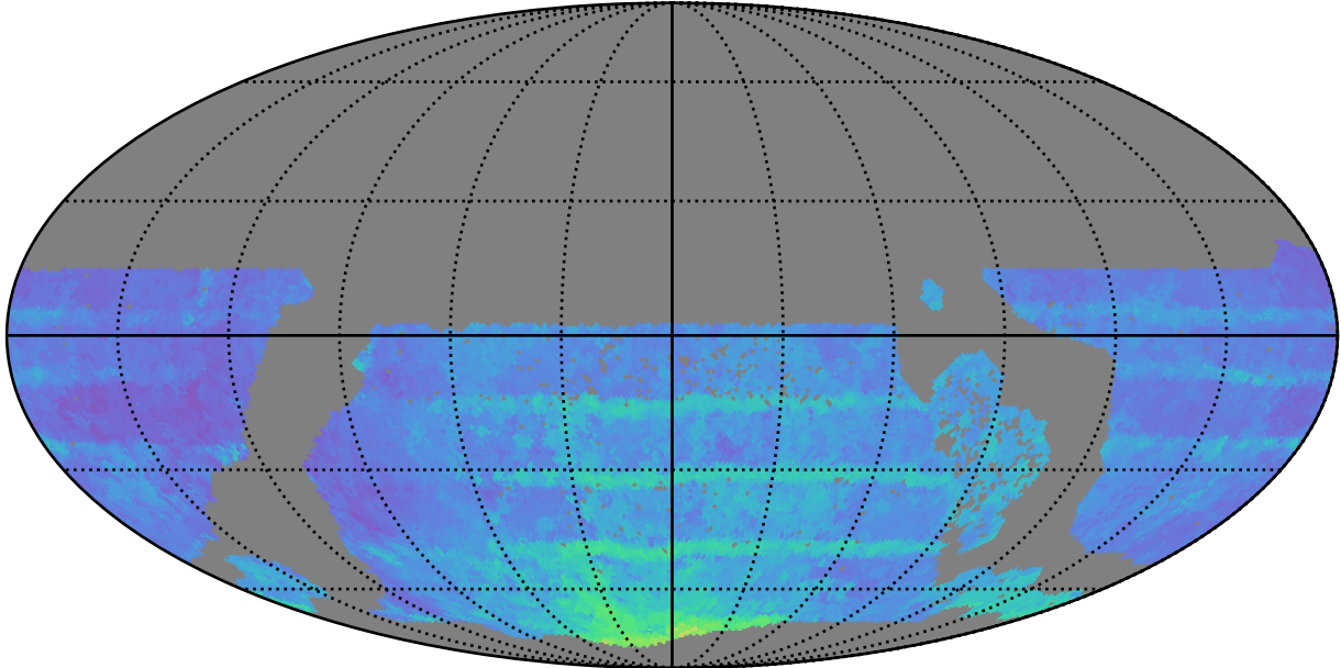
ddf_acor_sf30_lsf40_lsr50_v3.4_10yrs WFD all bands: 80thPercentile Season Length
