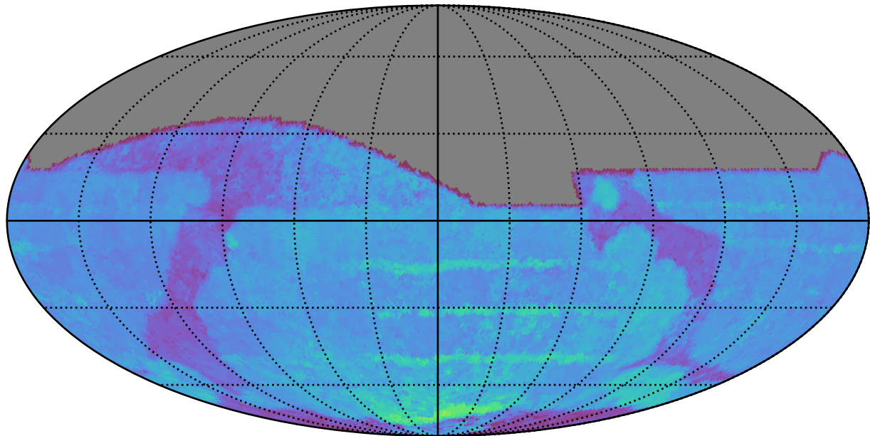
ddf_acor_sf30_lsf40_lsr50_v3.4_10yrs All sky i band: 80thPercentile Season Length
