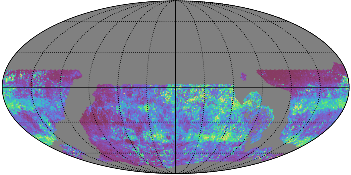
ddf_acor_sf30_lsf40_lsr50_v3.4_10yrs WFD zy bands: 75th Percentile Intranight Timespan
