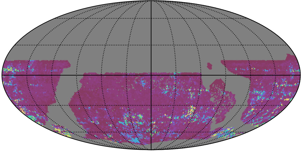
ddf_acor_sf30_lsf40_lsr50_v3.4_10yrs WFD z band: 75th Percentile Intranight Timespan
