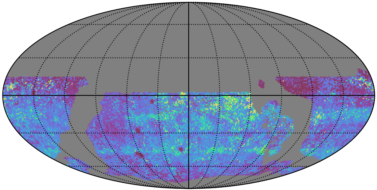
ddf_acor_sf30_lsf40_lsr50_v3.4_10yrs WFD y band: 75th Percentile Intranight Timespan
