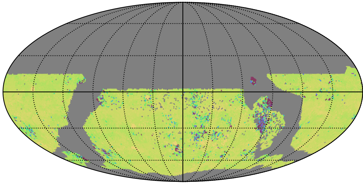
ddf_acor_sf30_lsf40_lsr50_v3.4_10yrs WFD ug bands: 75th Percentile Intranight Timespan
