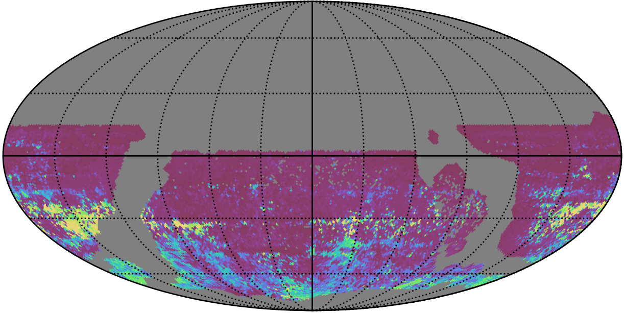
ddf_acor_sf30_lsf40_lsr50_v3.4_10yrs WFD r band: 75th Percentile Intranight Timespan
