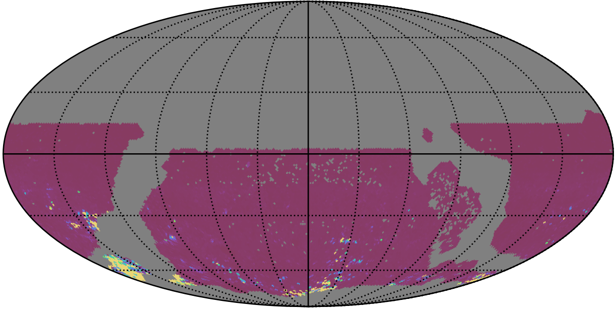
ddf_acor_sf30_lsf40_lsr50_v3.4_10yrs WFD gr bands: 75th Percentile Intranight Timespan
