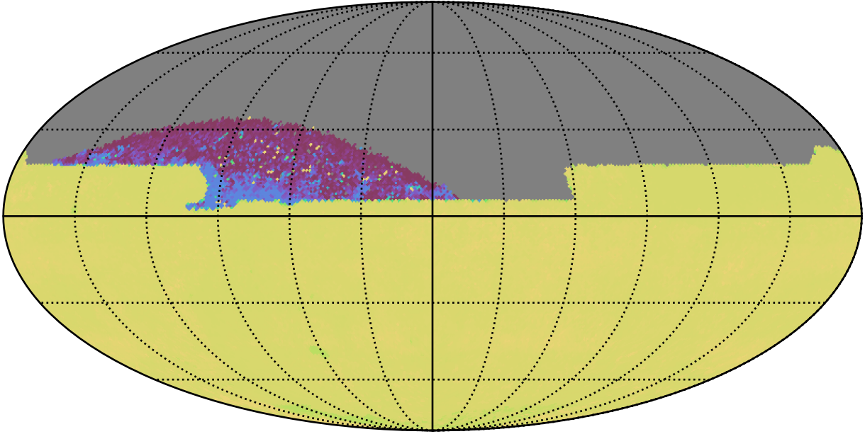
ddf_acor_sf30_lsf40_lsr50_v3.4_10yrs All sky zy bands: 75th Percentile Intranight Timespan
