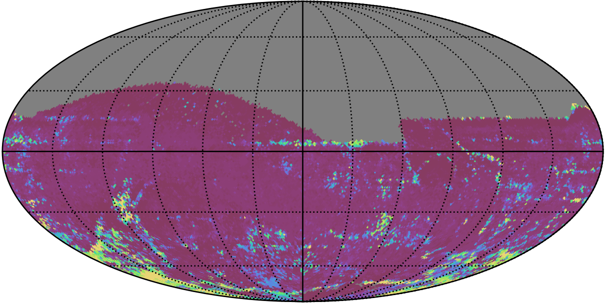
ddf_acor_sf30_lsf40_lsr50_v3.4_10yrs All sky z band: 75th Percentile Intranight Timespan
