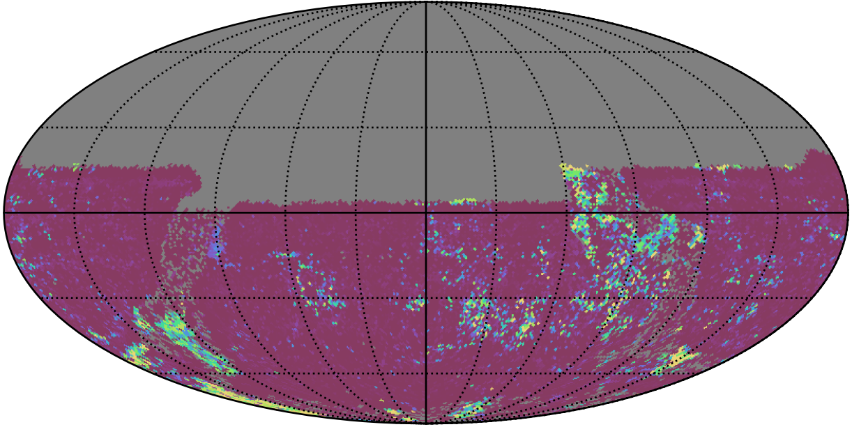
ddf_acor_sf30_lsf40_lsr50_v3.4_10yrs All sky u band: 75th Percentile Intranight Timespan
