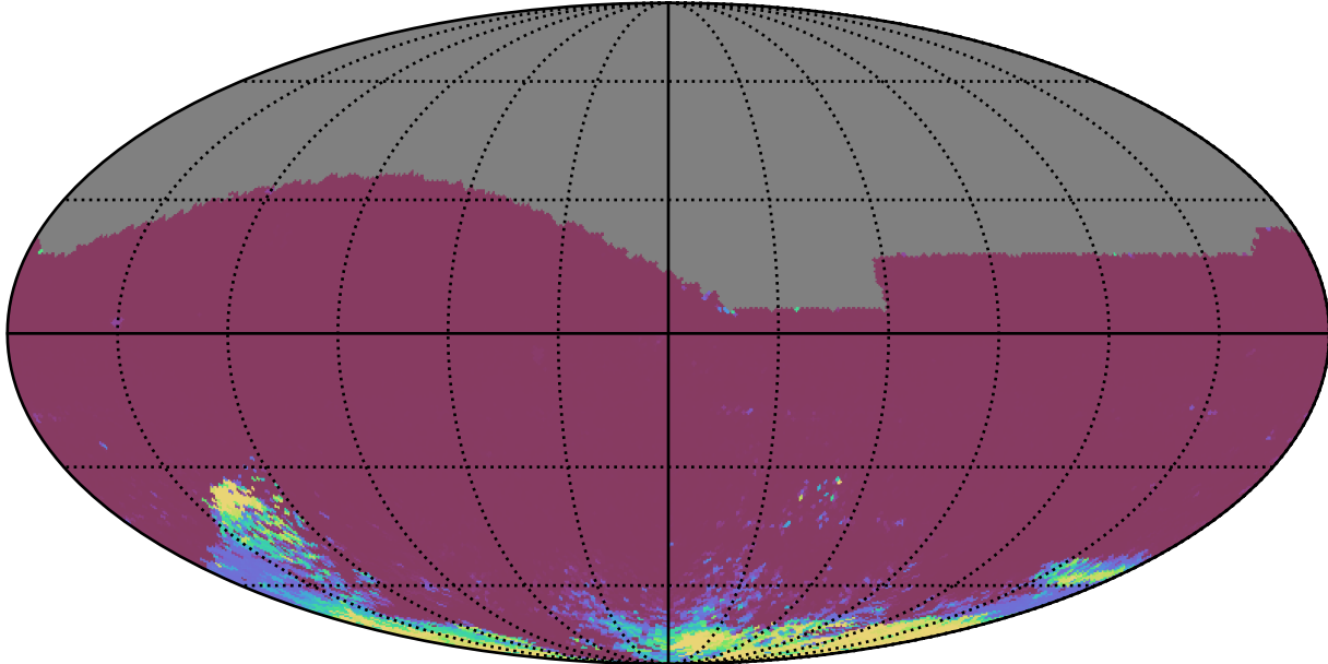
ddf_acor_sf30_lsf40_lsr50_v3.4_10yrs All sky ri bands: 75th Percentile Intranight Timespan
