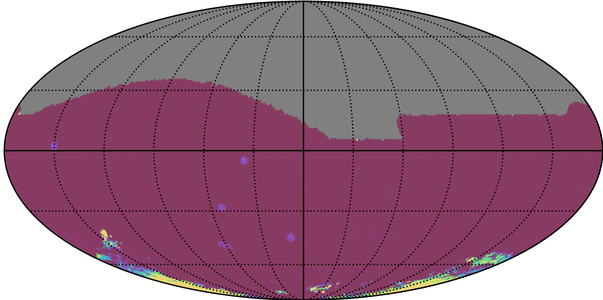
ddf_acor_sf30_lsf40_lsr50_v3.4_10yrs All sky iz bands: 75th Percentile Intranight Timespan
