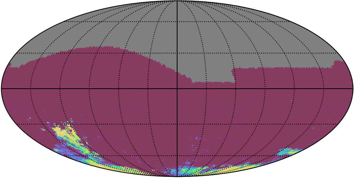
ddf_acor_sf30_lsf40_lsr50_v3.4_10yrs All sky gr bands: 75th Percentile Intranight Timespan
