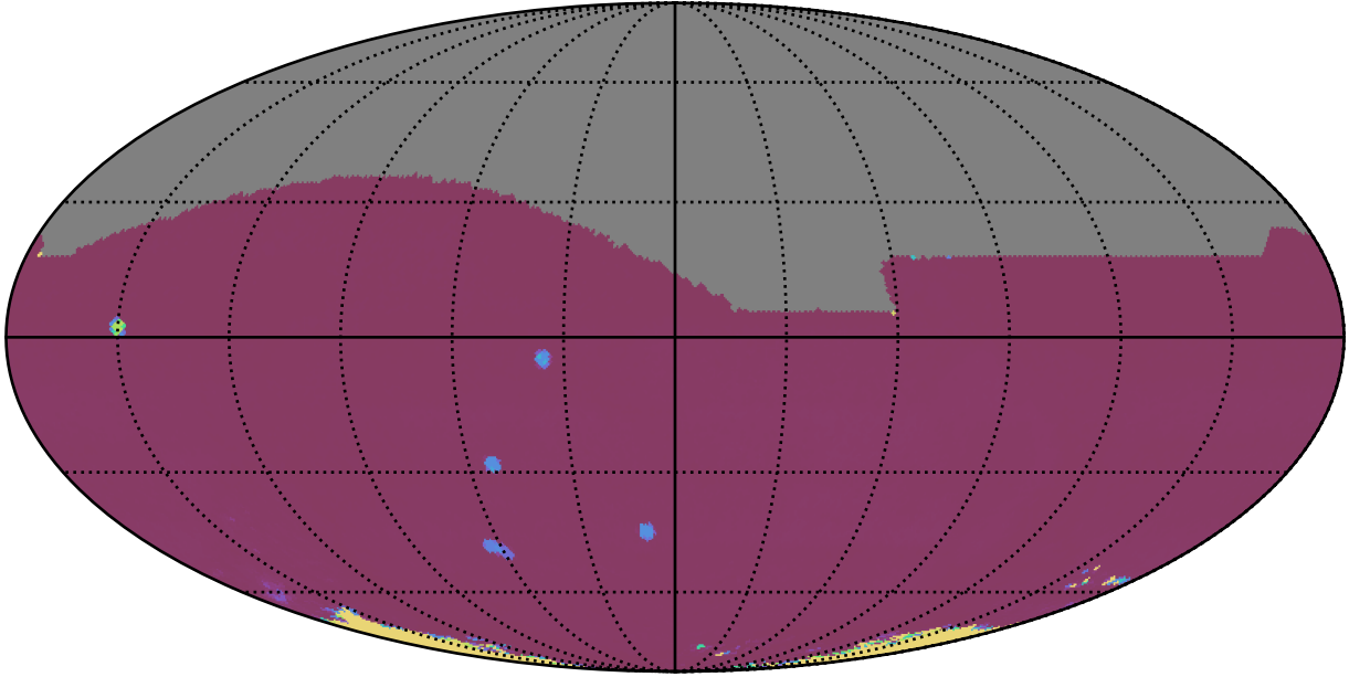
ddf_acor_sf30_lsf40_lsr50_v3.4_10yrs All sky all bands: 75th Percentile Intranight Timespan
