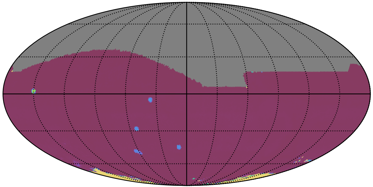
ddf_acor_sf30_lsf40_lsr50_v3.4_10yrs All sky: 75th Percentile Intranight Timespan
