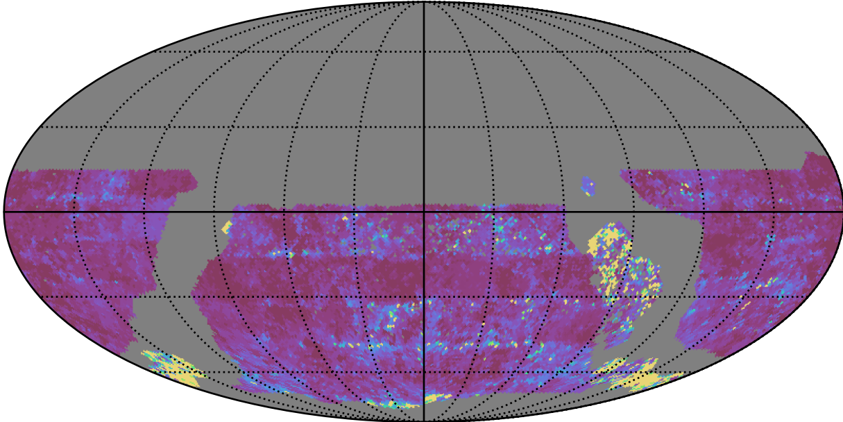
ddf_acor_sf30_lsf40_lsr50_v3.4_10yrs WFD u band: 20thPercentile Inter-Night Gap
